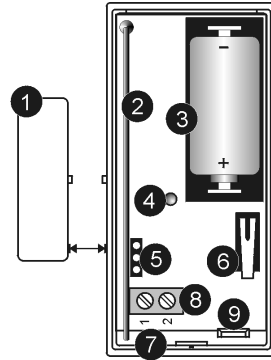
Figure 1: EL-2601 (cover off)/Figure 1: EL-2601 (sans couvercle) /Figure 1: EL-2601 (sin tapa)
